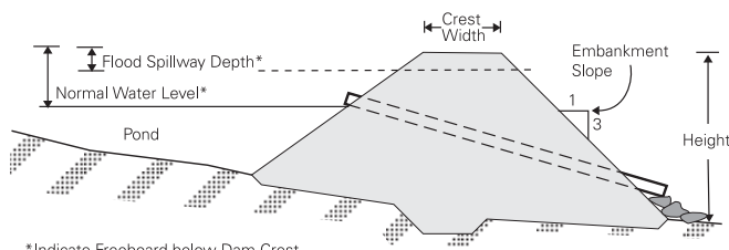
Cross Section of Dam
