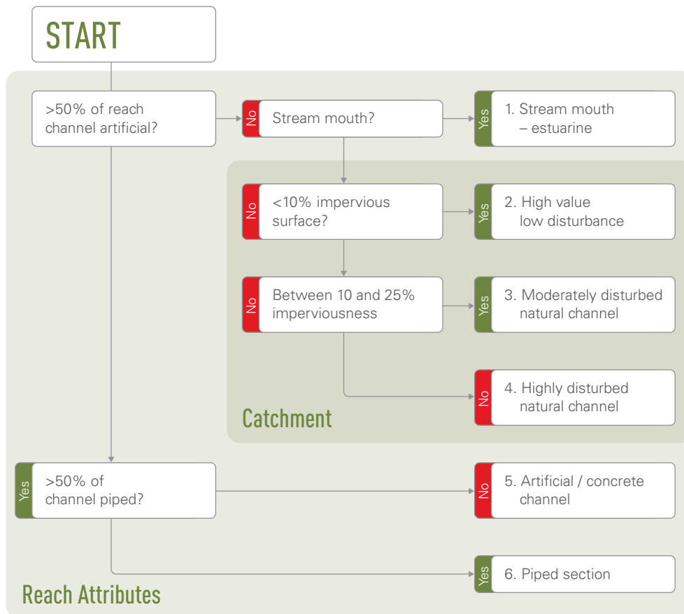
Figure 3.1 Flow Chart for Assigning Urban River and Stream Types Described in Section 3.6.2.2.
