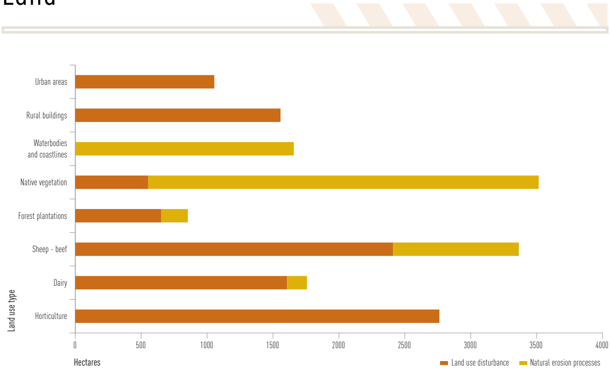
FIGURE 5 Hectares of bare soil and the proportions contributed by natural erosion and land use disturbance, by land use type. (Source: ARC).
