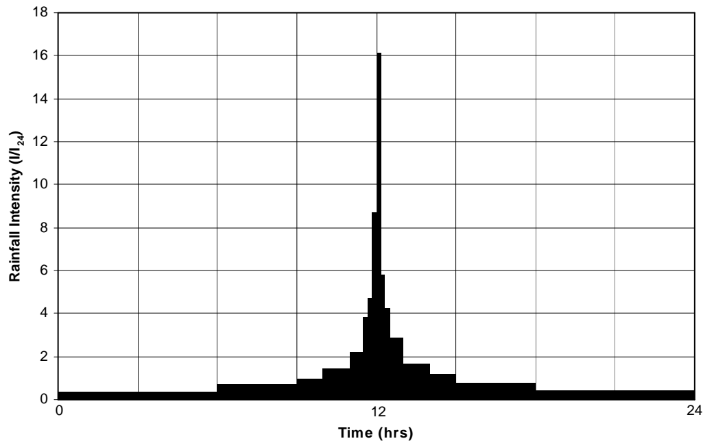
Figure 2.1 - Auckland Region 24 hour Design Storm
