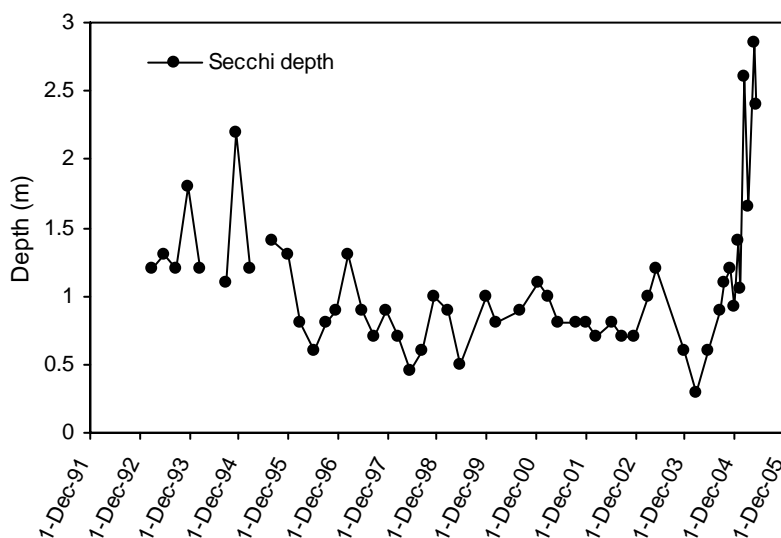
Figure 4.3: Secchi disc depths in Lake Wainamu (1992-2005).
