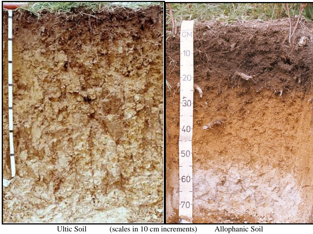
Figure 1. A low permeability, clayey Ultic Soil (left) compared with a moderate-to-high permeability, silty Allophanic Soil (right) on Waitemata Formation from the South Auckland area.
