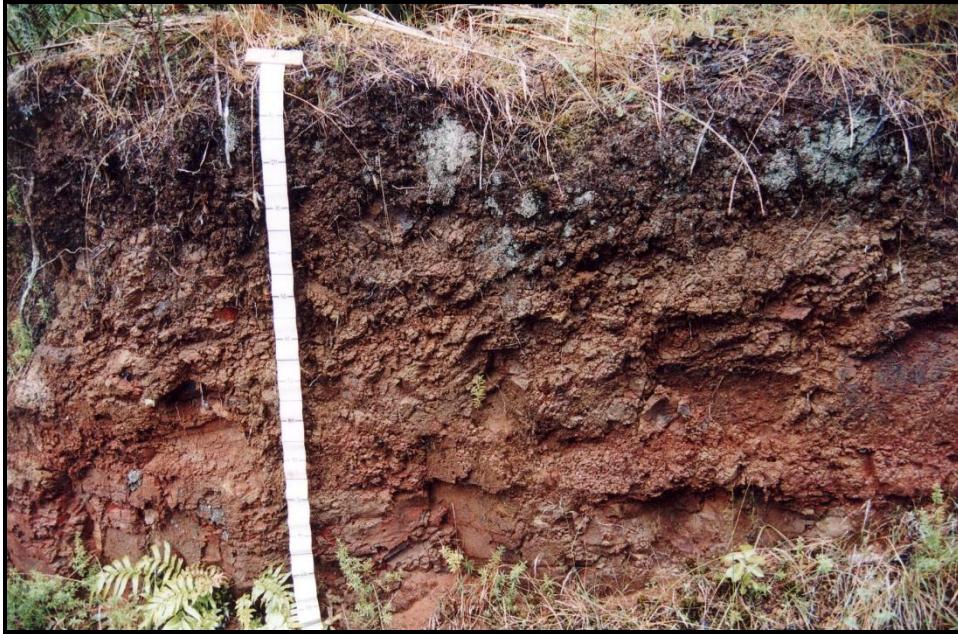
Figure 5. A high permeability Granular Soil from the Waitakere area. (scale in 10 cm increments)
